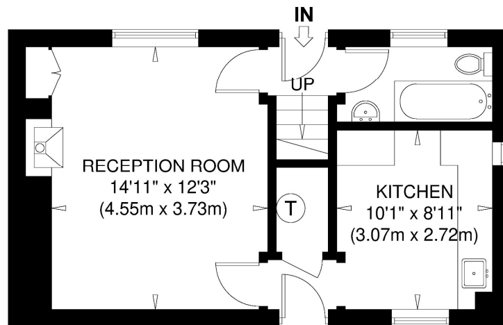
GROUND FLOOR GROSS INTERNAL FLOOR AREA 36.9 SQ M / 397 SQ FT
