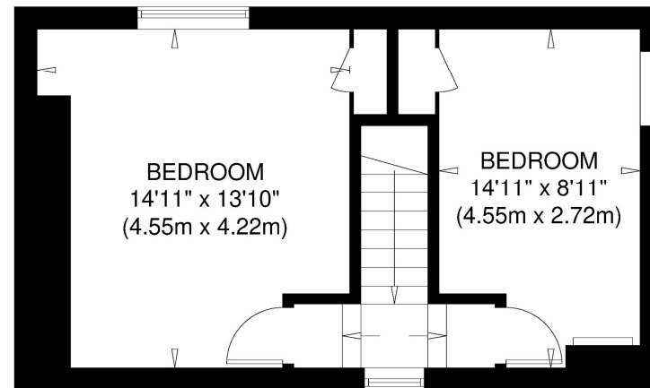
FIRST FLOOR GROSS INTERNAL FLOOR AREA 36.9 SQ M / 397 SQ FT
